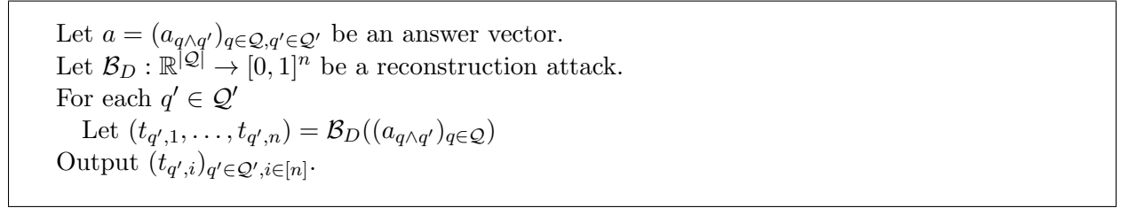
Figure 1: The reconstruction \mathcal{R}_D^*(a) .
